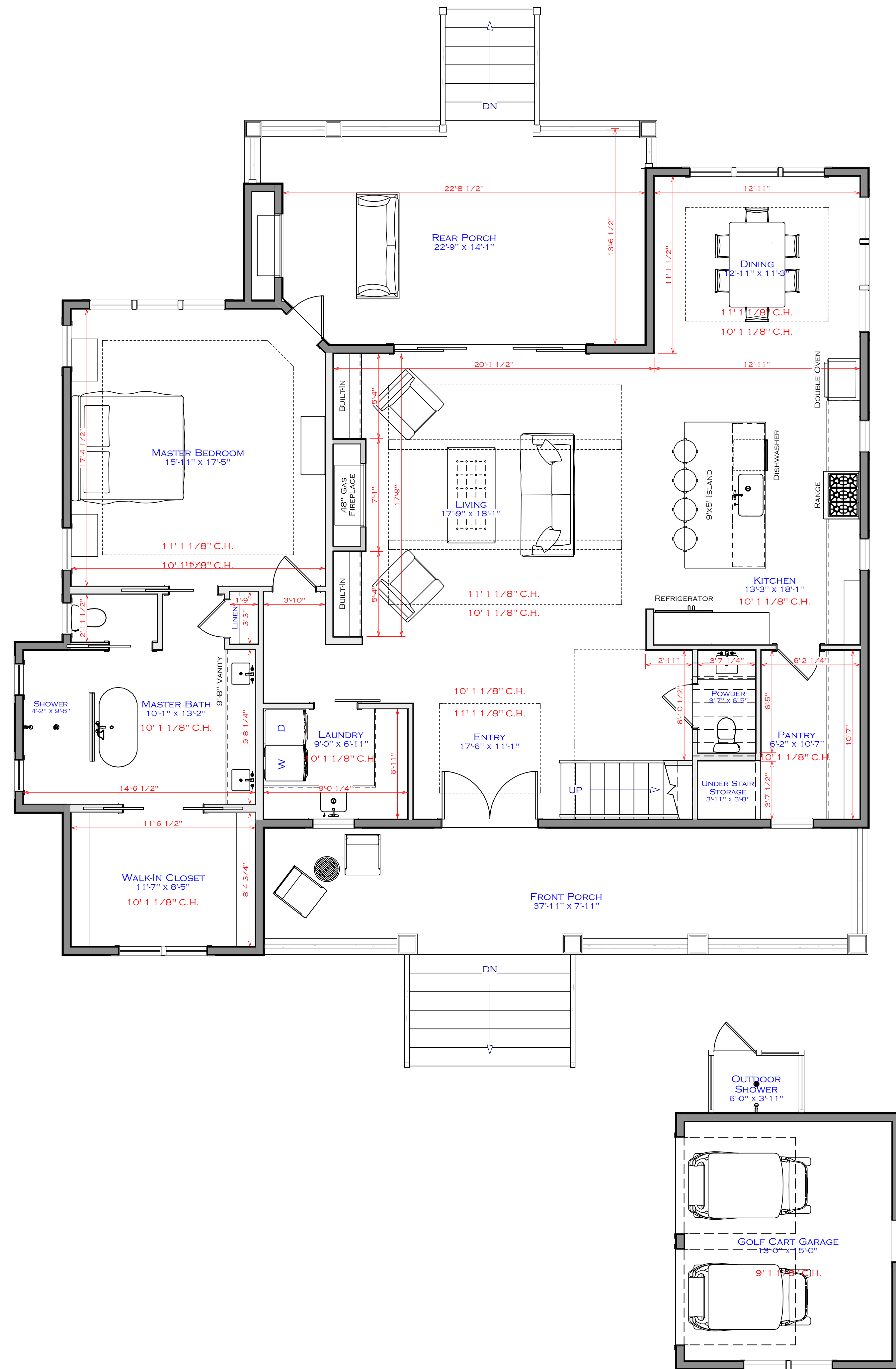
1 FURNITURE PLAN A-3 1/4" = 1'0"
