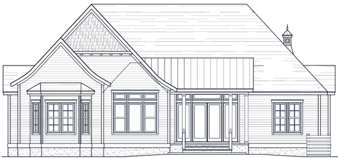
Rear Elevation
