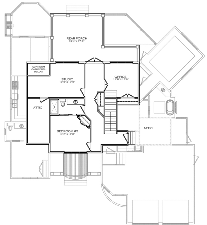
SECOND FLOOR
